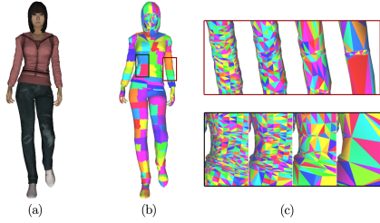
Figure 7: This figure shows an original model (a) and its leaf clusters generated by our error-aware clustering method (b). (c) show zoomed regions of boxed parts in (b). The top of (c) shows a deforming elbow region with increasing simplification levels. The bottom shows a non-deforming torso region, resulting in more aggressive simplification.
