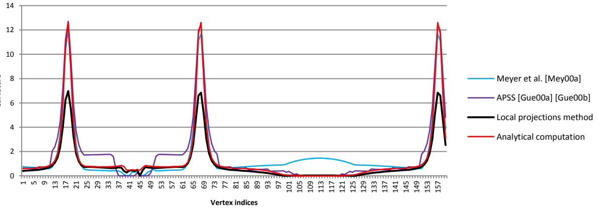
Figure 6. Surface z = \cos(x^2 + y^2) – maximum curvature
