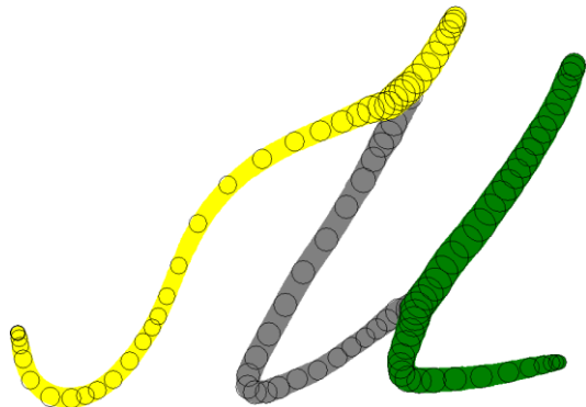
Figure 10. A step of "sewing" fat curves.
