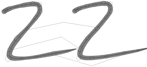
Figure 8. A smoothing of control-circle radiuses.
