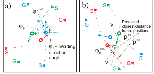
Figure 3: Avoidance scenarios illustrating the notations used in the text: (a) Angles \varphi_i, \varphi_i^{\text{goal}}, \varphi_{ij} shown for one character (blue). (b) Angle \varphi_{ij}^{\text{pc}} shown for one character (red). Crosses mark "Start" and "Goal" positions for the characters
