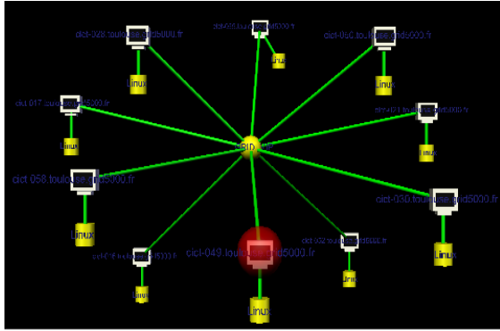
Figure 4: Event display
