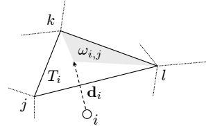
Figure 2: The element h_{ij} provides the barycentric coordinate \omega_{i,j} of the contact point i projected onto the penetrated surface triangle T_i with respect to j \in T_i .
