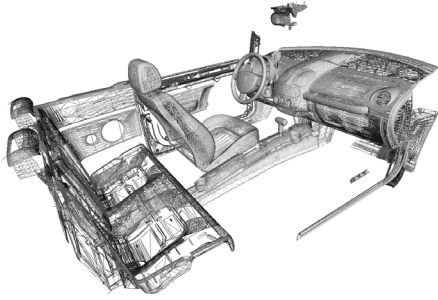
Figure 8. Tessellation of the Beetle interior.
