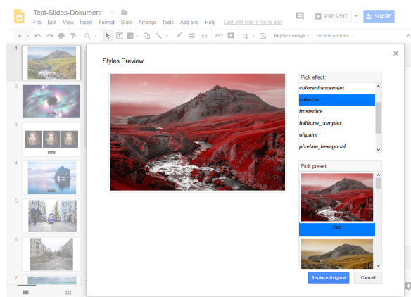
Figure 4: Example of the integration of service-based image-abstraction techniques into Google Slides via an Add-on using server-sided Google Script.
