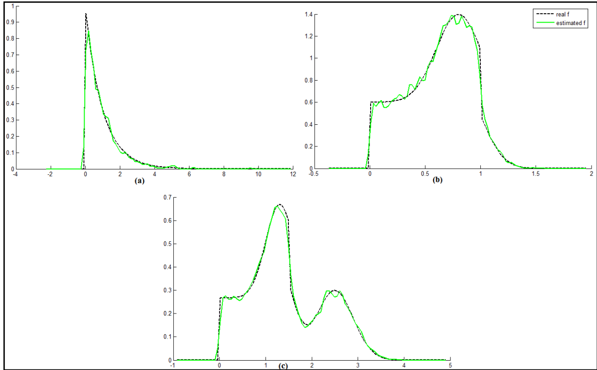
Figure 1: Estimation of the three distributions by the conventional kernel method: (a) the exponential distribution \exp(x) , (b) the first mixture and (c) the second mixture.
