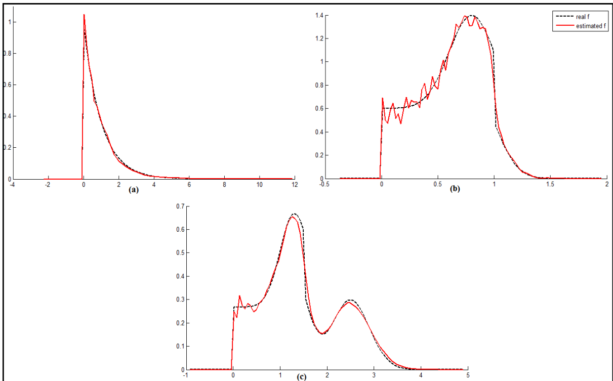
Figure 3: Estimation of the three distributions by the FSKDP: (a) the exponential distribution \exp(x) , (b) the first mixture and (c) the second mixture.
