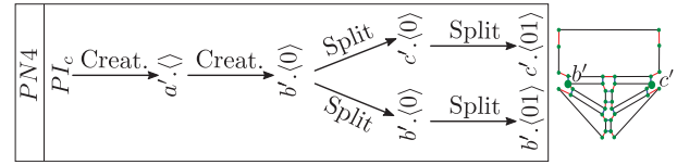
Figure 13: After 3-Triangulation.
