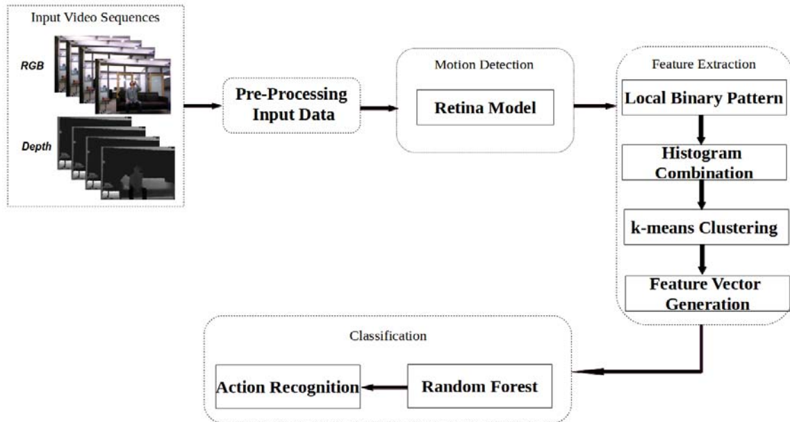
Figure 1: General structure steps of our approach for action recognition using RGB and depth video. Pre-Processing to the input video data, Motion detection, Feature extraction, and Classification.
