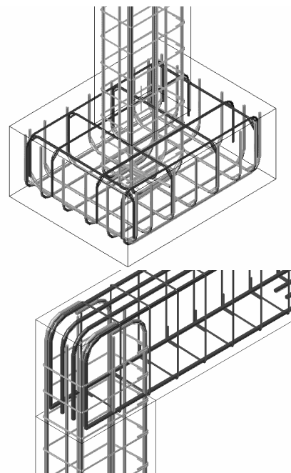
Figure 9: Complex relationship between reinforcements in the joint zones of the structural elements.
