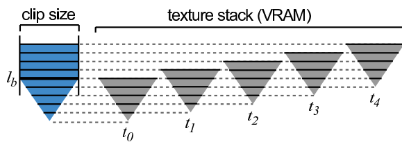
Figure 2: Texture stack.
