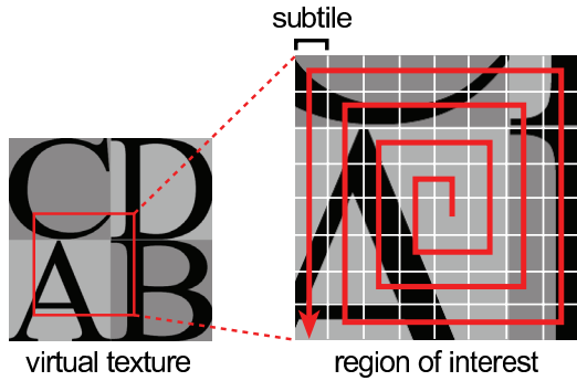
Figure 6: Circular update.
