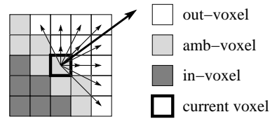
Figure 12: Normal estimation from voxels.
