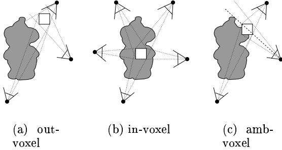
Figure 2: Voxel classification.
