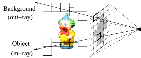
Figure 4: Pixel-rays.
