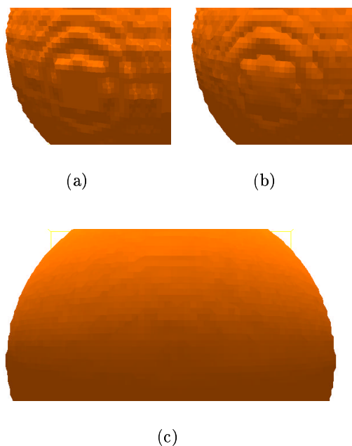
Figure 15: Rendering using voxel normal: in a voxel, all the triangles normals are replaced by the voxel normal. a. with edges-centers Marching cubes; b. with pixel-rays; c. with smoothed normal (distance of 5 voxels).
