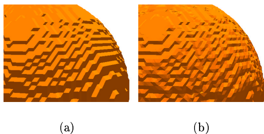
Figure 13: Rendering using triangles; a. with edges-centers marching cubes; b. with pixel-rays marching cubes.
