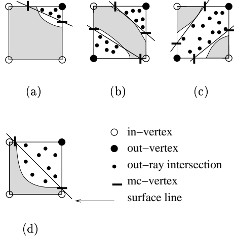
Figure 8: Intersection between out-rays and voxel faces - several cases; a. for usual cases; b. & c. with a disconnected surface; d. voxel vertices used as a boundary.
