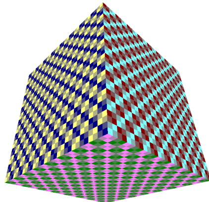
Figure 7: Cube texture
