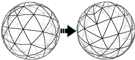
Figure 5: Parametrizations
